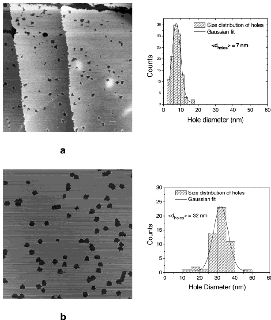
Figure 1. STM images of two HOPG surfaces modified by one-atomic-layer-deep holes with diameters of (a) 7 and (b) 32 nm. Image size: (a) 400 \times 400 \text{ nm}^2 and (b) 800 \times 800 \text{ nm}^2 .
