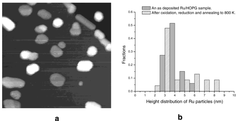
Figure 8. (a) STM image of the Ru/HOPG sample (15 atom % Ru) after the oxidation and reduction treatment. Image size: 200 \times 200 nm 2 . (b) The height distributions of the Ru/HOPG sample before and after the oxidation and reduction.
