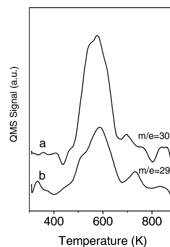
Figure 11. ^{15}N_2 (a) and ^{15}N^{14}N (b) TPD spectra from a Ru/HOPG sample ( \sim 10 atom % Ru) first exposed to ^{15}N_2 ( 2 \times 10^5 L) and then to ^{14}N_2 ( 4 \times 10^4 L) at 400 K.
