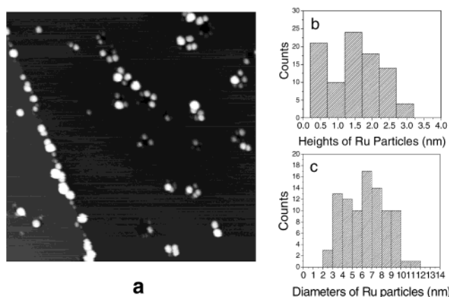
Figure 2. (a) STM image of a small hole-modified Ru/HOPG surface (2 atom % Ru). Image size: 200 \times 200 \text{ nm}^2 . (b) Height and (c) diameter distributions of the Ru particles in (a).
